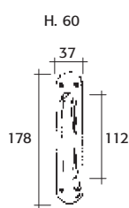
Martellina placca lucida Window handle polished plates art. 987-EL/Ø 7 OV-OB 4
