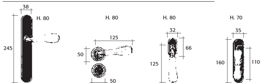
Martellina Window handle
