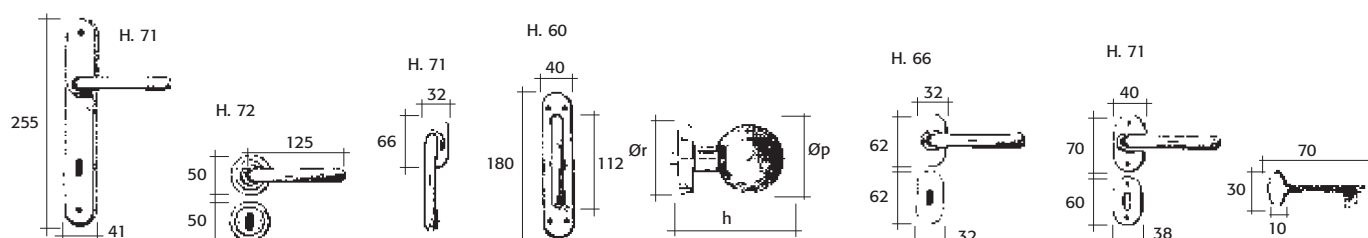
Martellina placca satinata Window handle art. 987/Ø 7
